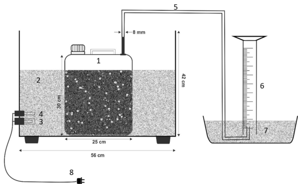
Fig. 2 Structural design of thermophilic biogas digester
